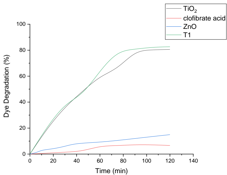
Figure 5. Degrivation of clofibrate acid using deferent time of irradiation in presence of ZnO NPs
