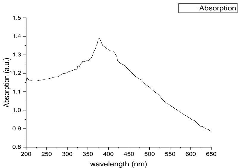
Figure 4, UV-Vis spectrum of ZnO nanoparticles
