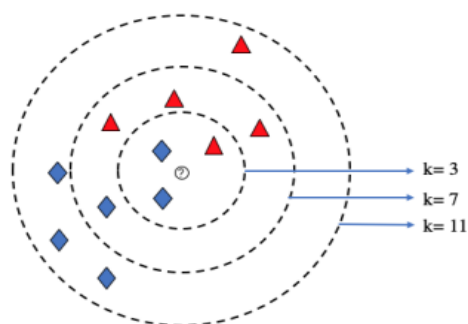
Fig. 2. K-nearest Neighbor
