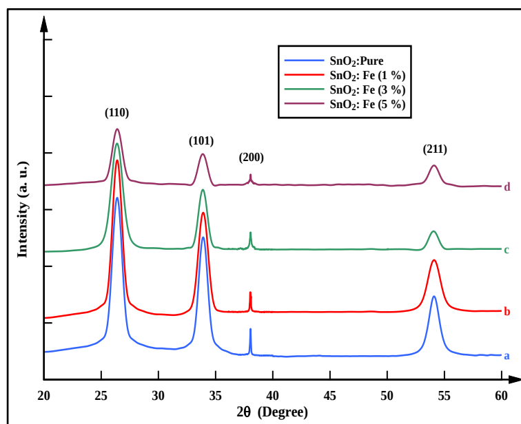
Figure (1): XRD pattern of \text{SnO}_2 : Fe thin films with different volume percentage of Fe; (a)- pure \text{SnO}_2 , (b)- 1% Fe, (c)- 3 % Fe and (d)- 5 % Fe
