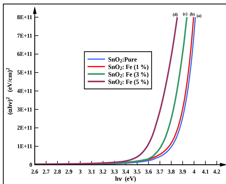
Figure (6): Energy gap of of (a) \text{SnO}_2 , (b) \text{SnO}_2 :1% Fe, (c) \text{SnO}_2 :3 % Fe and (d) \text{SnO}_2 :5 % Fe
