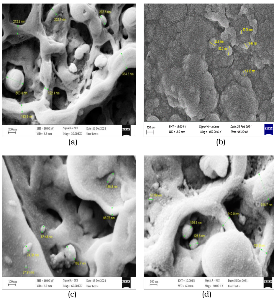
Figure (3): SEM images of (a)- pure \text{SnO}_2 , (b)- \text{SnO}_2\text{: 1% Fe} , (c)- \text{SnO}_2\text{: 3% Fe} and (d)- \text{SnO}_2\text{: 5% Fe} .
