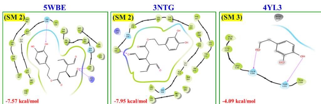
Fig. 3. Two-dimensional representation of selected small molecules with the amino acids present in the catalytic site of anti-inflammatory molecular target
