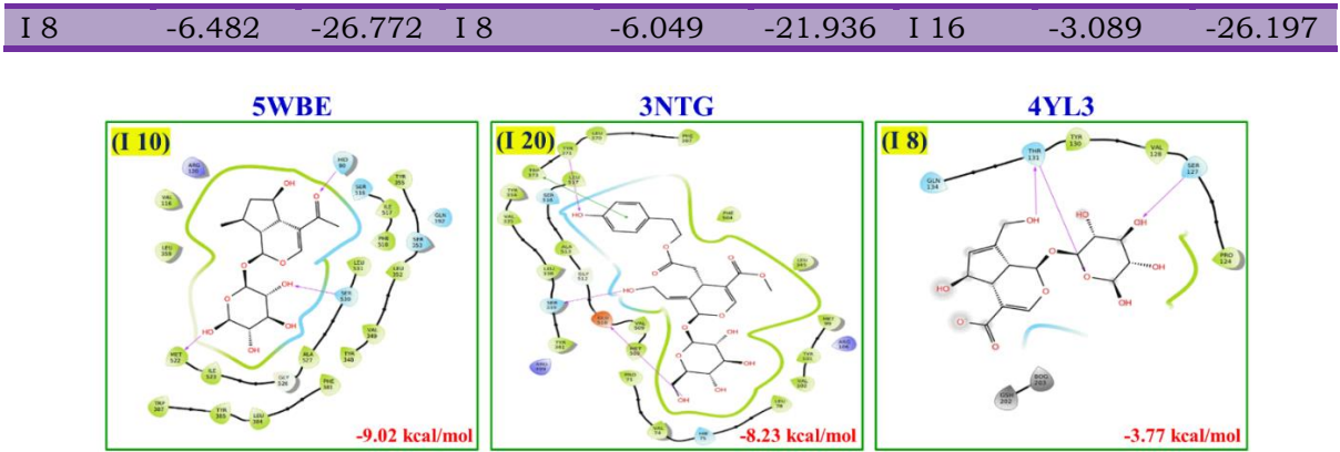
Fig. 2. Two-dimensional representation of selected iridoids with the amino acids present in the catalytic site of anti-inflammatory molecular target
