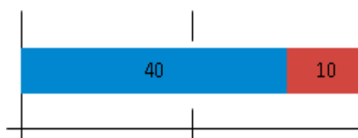
Figure 2-Gender wise distribution
