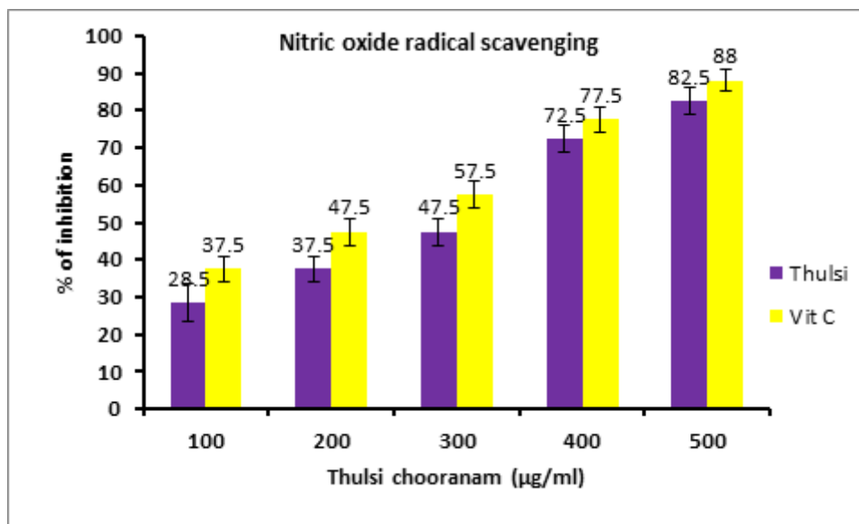
Figure 5-shows Nitric oxide radical scavenging between Thulsi and VitaminC
