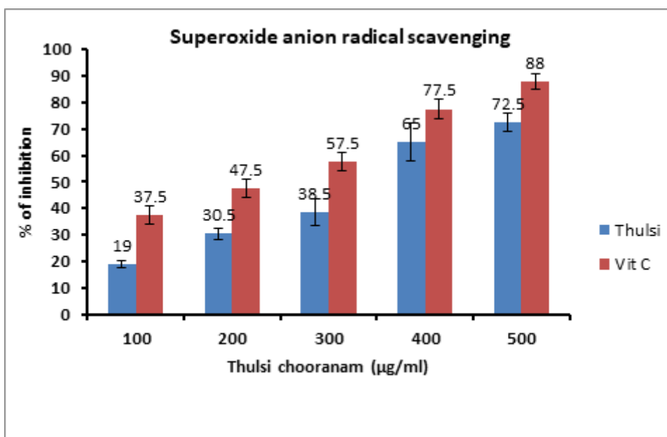
Figure 4-shows the results of Superoxide anion radical scavenging between Thulsi and VitaminC
