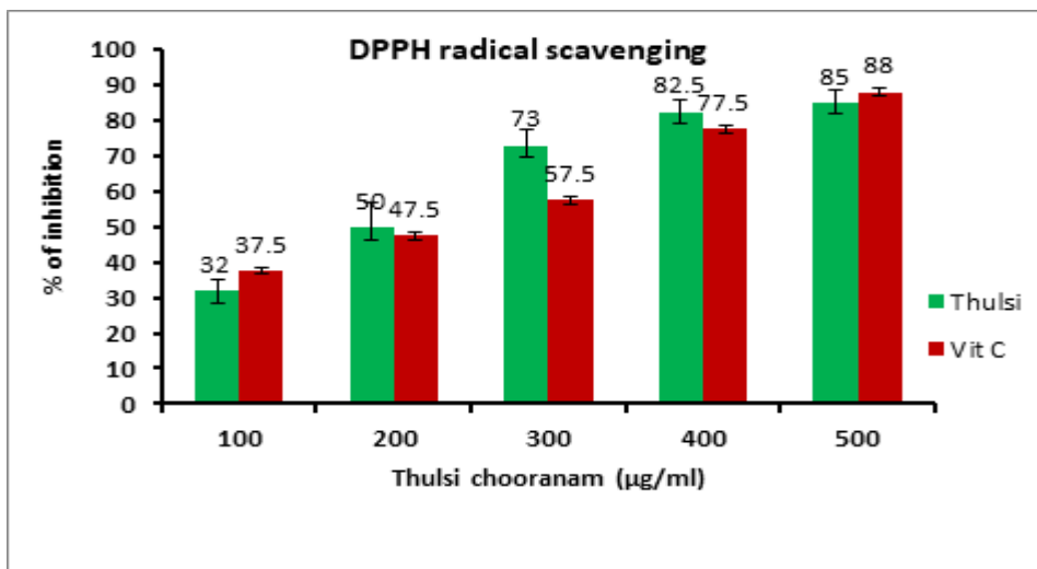
Figure 3-shows in DPPH radical scavenging between Thulsi and VitaminC
