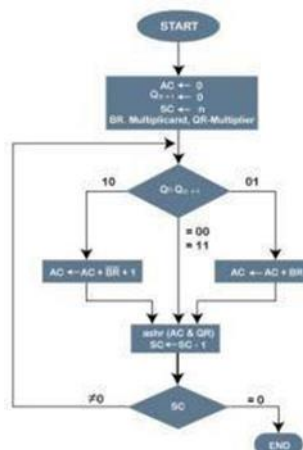
Figure 7 Booth Multiplier
