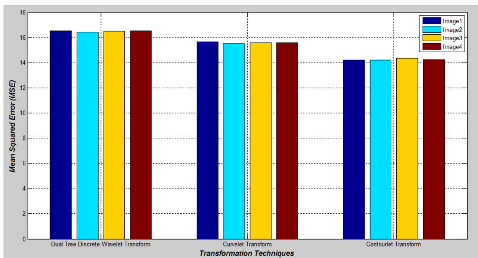
Figure 2: Performance analysis of the transformation techniques like Dual Tree Discrete Wavelet Transform, Curvelet Transform, and Contour Transform against Mean Squared Error (MSE)
