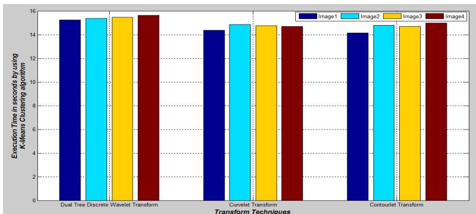
Figure 4a: Performance analysis of the K-means segmentation algorithm by using different transform techniques against execution time
