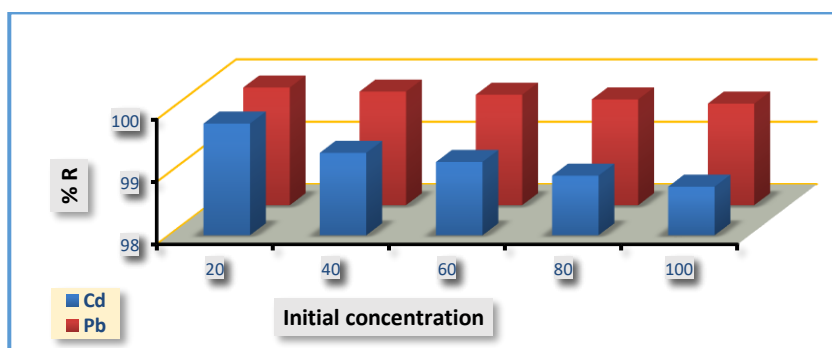
Fig.9.effect of the initial concentration of ions (Pb, Cd) on the percentage of their removal
