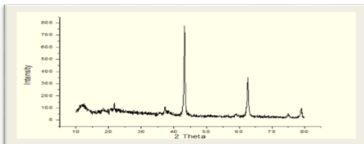
Fig.3.XRD diagram of MgO NPs prepared using green tea extract
