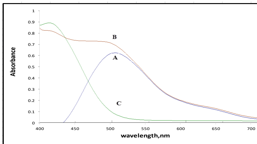
Fig. 6: Absorption spectra of 100 ppm CFX treated according to the recommended procedure against (A) blank, (B) distilled water and (C) blank measured against distilled water
