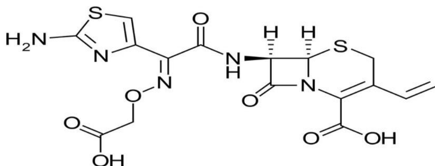
(CFX) (C 16 H 15 N 5 O 7 S 2 ) M.wt.= 507.5 g/mol
