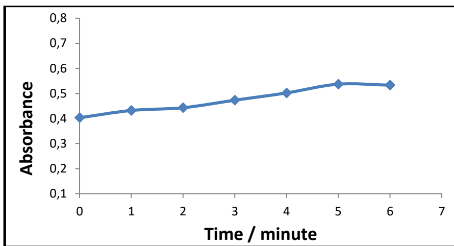
Fig. 2: Effect of time on the diazotization reaction
