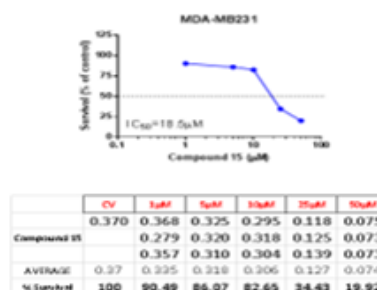
Figure (20) Results obtained for measuring the IC 50 of copper complex
