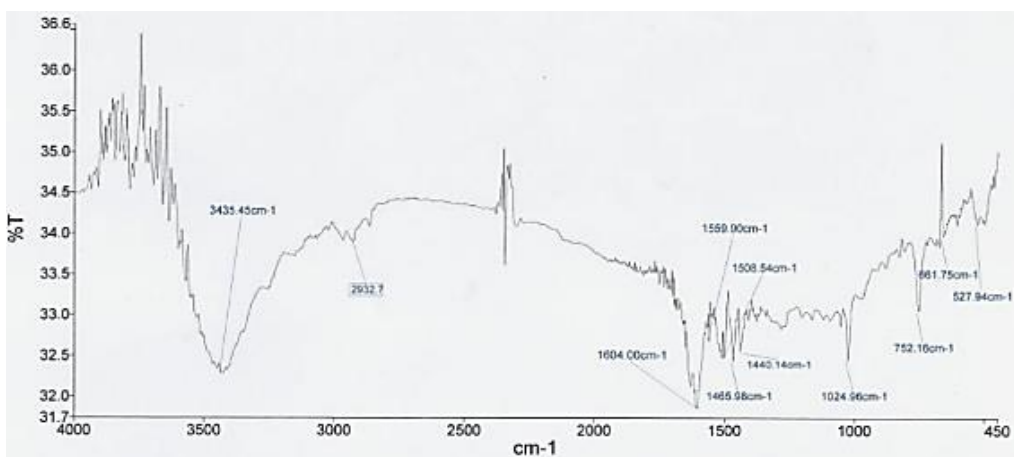
Figure (10) Infrared spectrum of Cu(L) complex.
