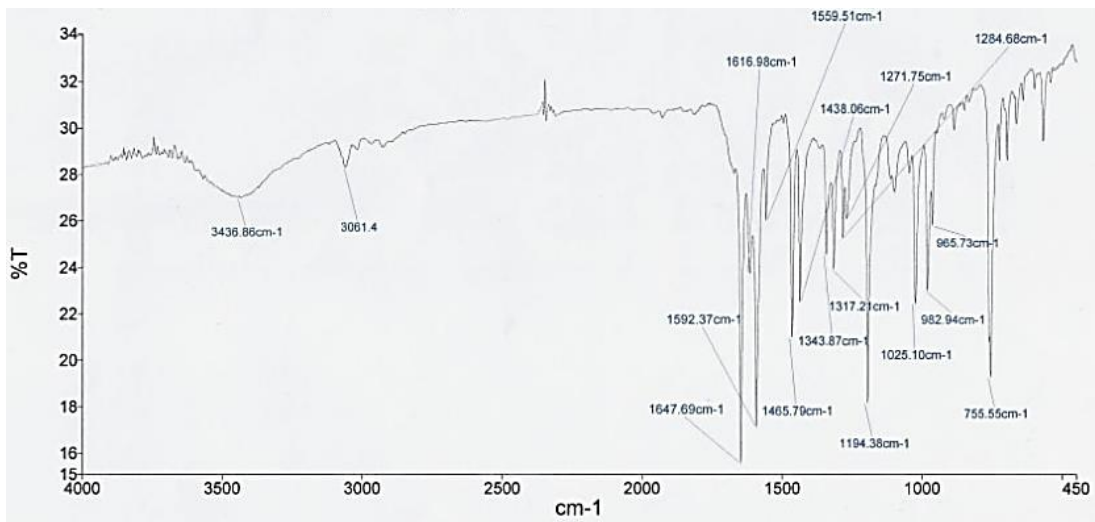
Figure (7) Infrared spectrum of the compound D-o-Br-BA.
