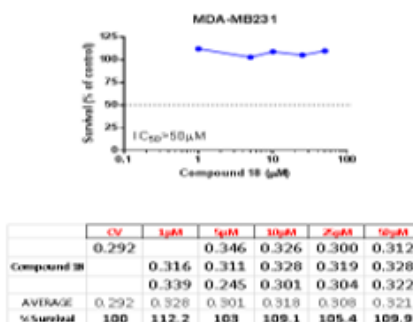
Figure (21) The results obtained for measuring the IC 50 of iron complex.
