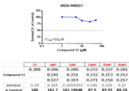
Figure (19) Results obtained for measuring the IC 50 of the nickel complex
