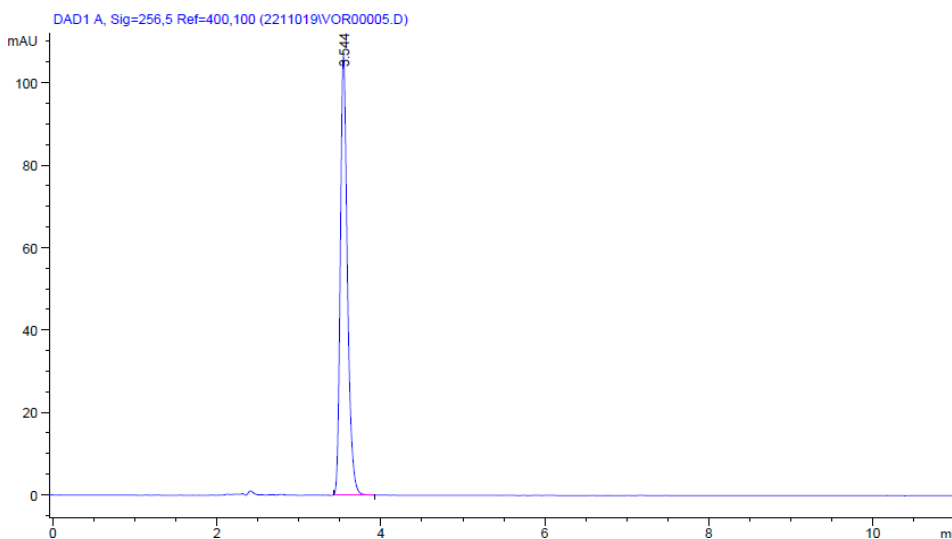
Fig. 1 Standard chromatogram of voriconazole (20 \mu\text{g/ml} )
