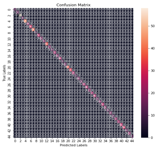
Figure 4. Confusion Matrix
