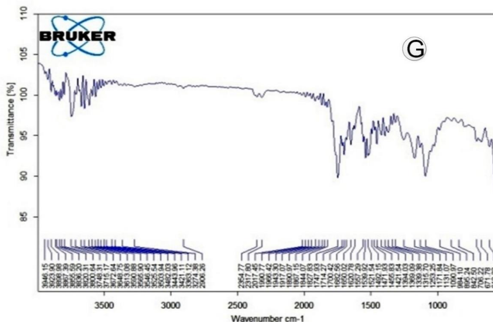
Figure 1. Fourier transform infrared (FTIR) spectra of drug with excipients (Paclitaxel, PLGA, PVA, Soluplus®, FOL)
