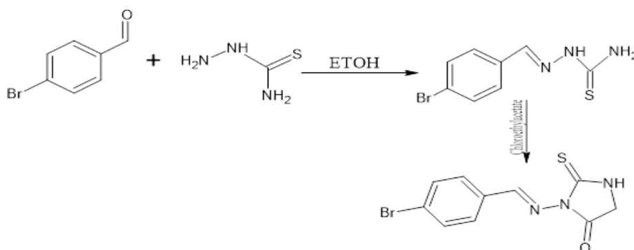
Scheme (1): Synthesis of Ligand (L)
