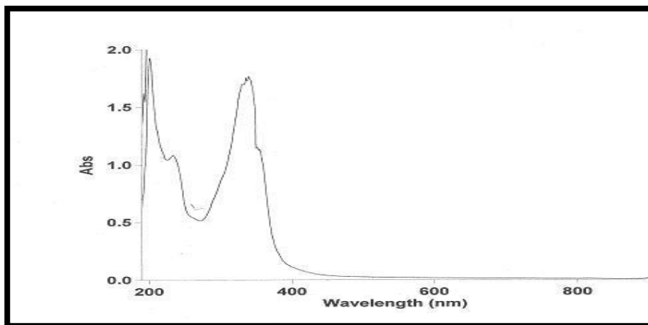
Figure (3-5) U.V spectrum of ( L)
