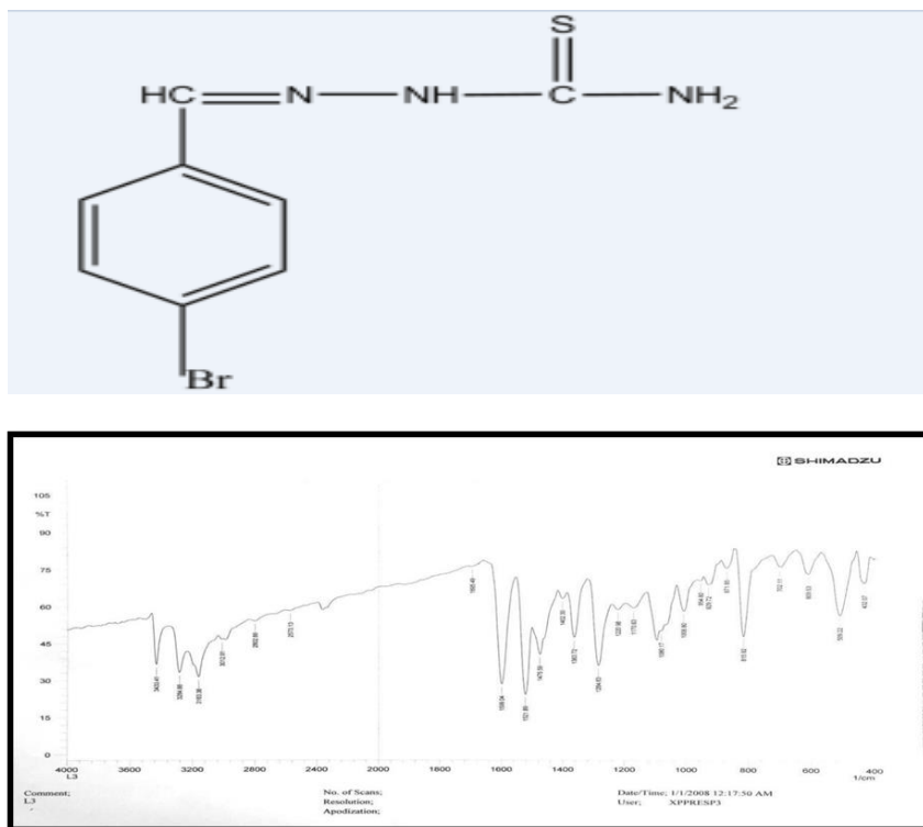
Figure(3-1) FTIR spectrum of compound (A).
