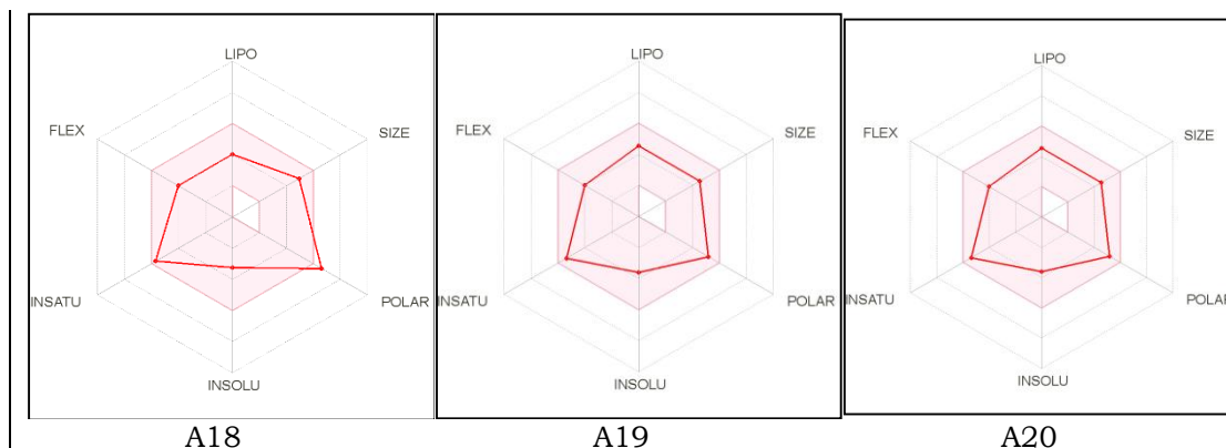
Figure 3. The coloured zone is the acceptable physicochemical area for oral bioavailability, according to the physicochemical radar of the molecules. Where, LIPO (Lipophilicity): -0.7 < XLOGP3 < +5.0 , SIZE: 150 \text{g/mol} < MV < 500 \text{g/mol} , POLAR (Polarity): 20 \text{\AA}^2 < TPSA < 130 \text{\AA}^2 , INSOLU (Insolubility): 0 < \text{LogS (ESOL)} < 6 , INSATU (Instauration): 0.25 < \text{Fraction Csp3} < 1 , FLEX (Flexibility): 0 < \text{Num. of rotatable bonds} < 9
