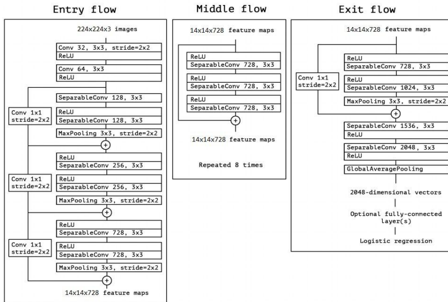
Figure 3. Xception network
