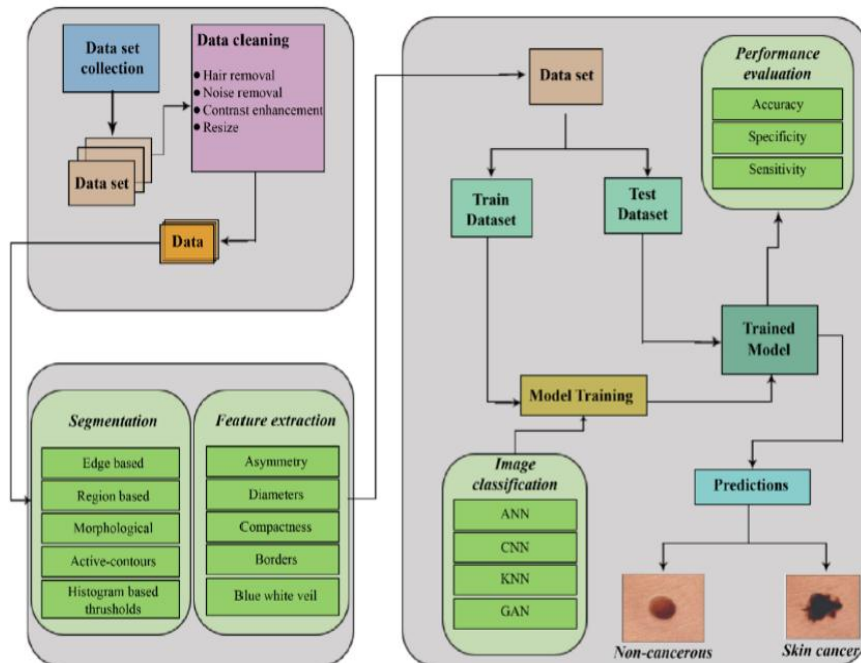
Figure 4. Skin Cancer Detection Process
