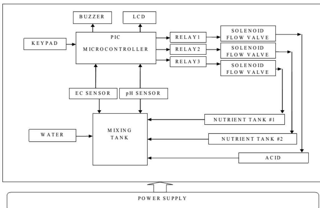
Fig.8: Components of automatic fertigation system.
