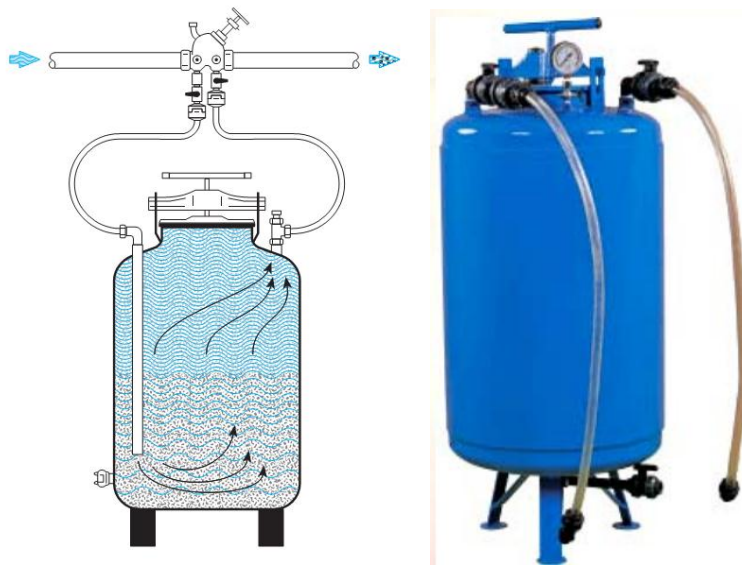
Fig.2: Pressure differential tank.
