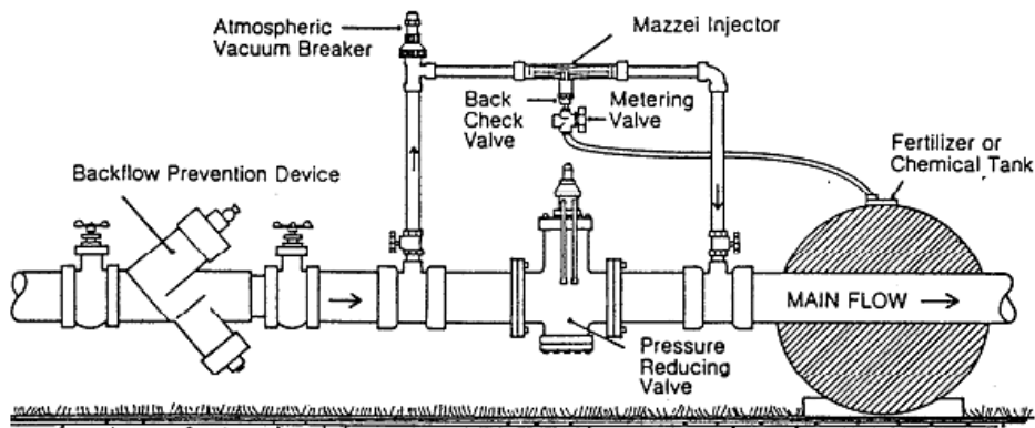
Fig.1: Fertigation system components connected to the irrigation system main line.
