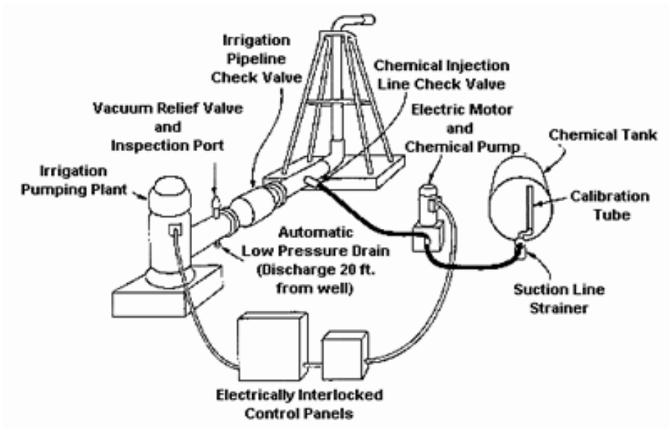
Fig.7: Interlock devices.
