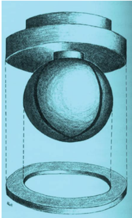
Figure 3. Resilient attachment
