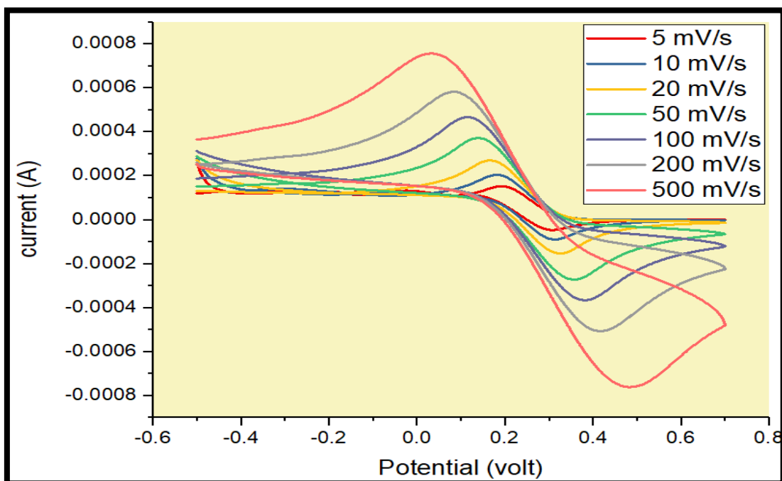
Fig.1 (A) Cyclic voltammograms of 5 \times 10^{-3} mM K_3 [Fe (CN) _6] at scan rates of (1)5, (2)10, (3)20, (4)50, (5) 100 (6)200 (7)500 mV/s.
