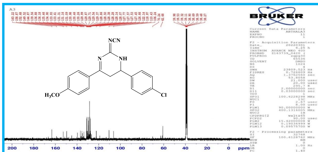
Figure 6. The 13 C-NMR spectrum of compound (I16)
