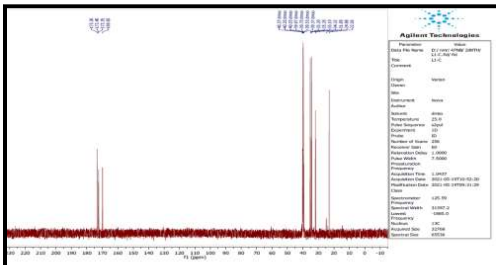
Fig (2): ^{13}\text{C} -NMR spectrum for ligand(ATA)
