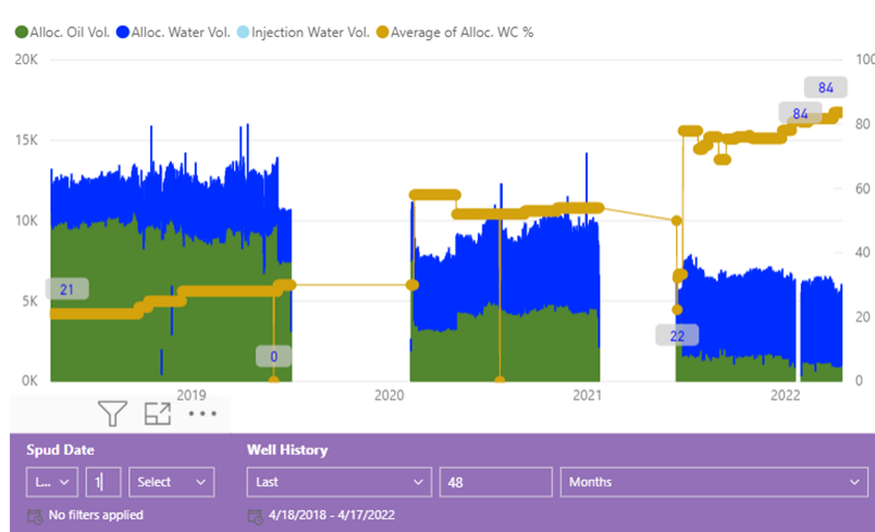
Figure (1-1) Well X2 Production History
