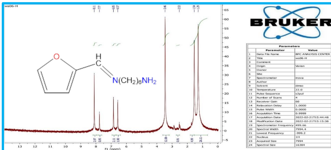
Figure 2: 1 H-NMR spectrum of WS.X1
