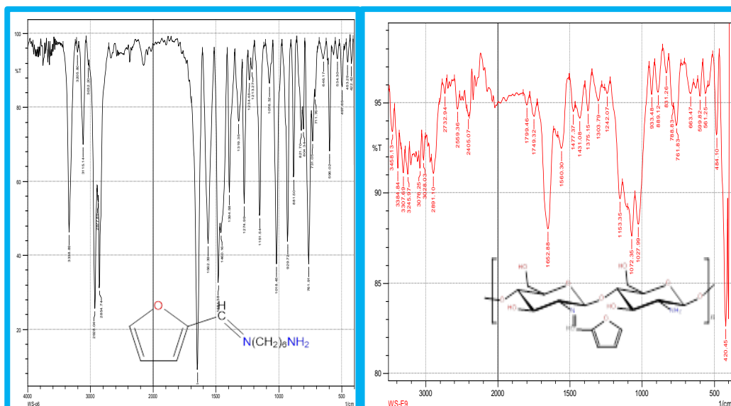
Figure 1: FTIR spectrum of WS.X1 and WS.X5
