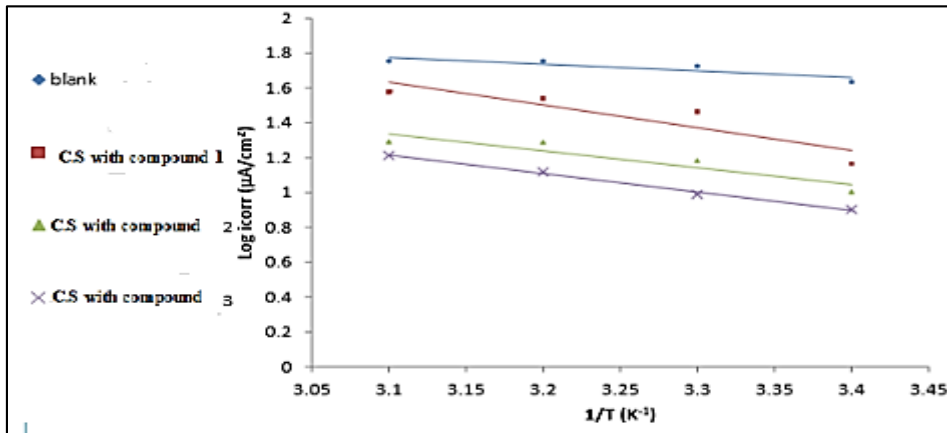
Figure 11-Plot of \log i_{corr} vs. 1/T for the compounds(B1-B3) in the absence and presence of the inhibitors in 3.5% NaCl solution.
