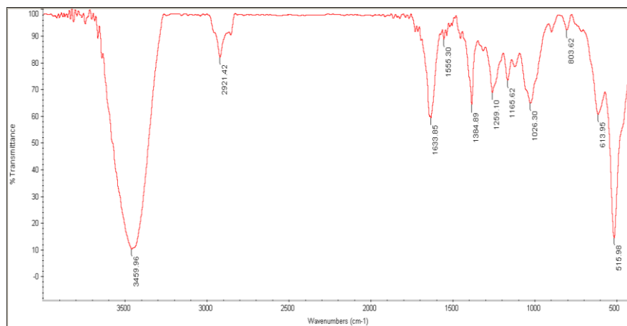
Figure (4) Examination of the nanomaterial (reduced graphene oxide and nano-chitosan)
