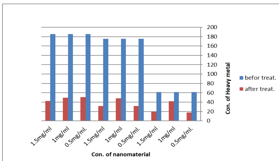
Figure (6) The results of the effectiveness of the nanomaterial (reduced graphene oxide and nano-chitosan) at a concentration (0.5,1,1.5 mg/ml) in removing Lead at a concentration (0.1,0.2,0.3 mg/ml) in (24h)
