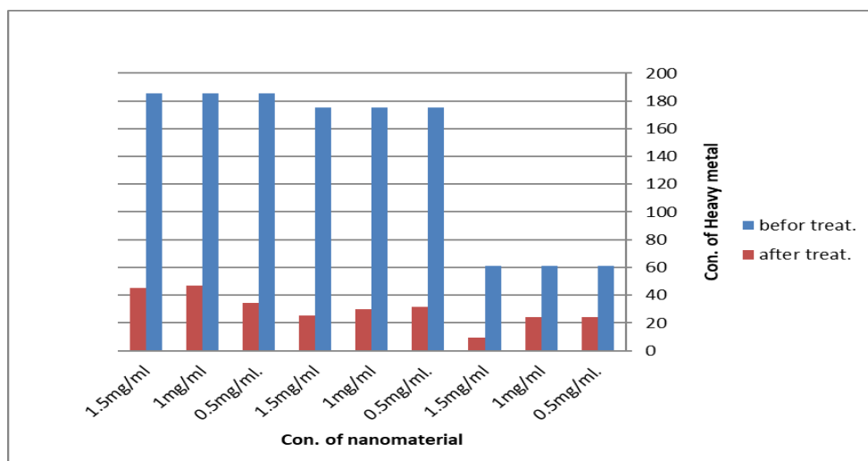
Figure (7) The results of the effectiveness of the nanomaterial (reduced graphene oxide and nano-chitosan) at a concentration (0.5,1,1.5 mg/ml) in removing Lead at a concentration (0.1,0.2,0.3 mg/ml) in (48h)
