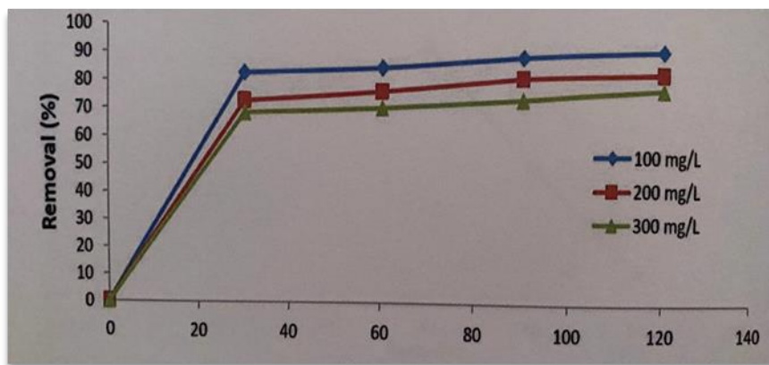
Figure (10) Shows the effect of contact time on the percentage of nickel ions removal using copper oxide CuO nanoparticles with different initial concentrations (Hassan and Mahadi, 2017).
