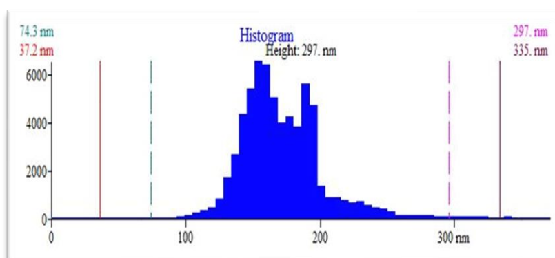
Figure (3) Atomic force microscopy analysis of the nanomaterial (reduced graphene oxide and nano-chitosan)
