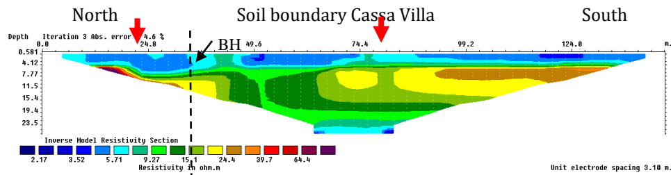
Figure 3. Cross-sectional resistivity contour of a measurement
